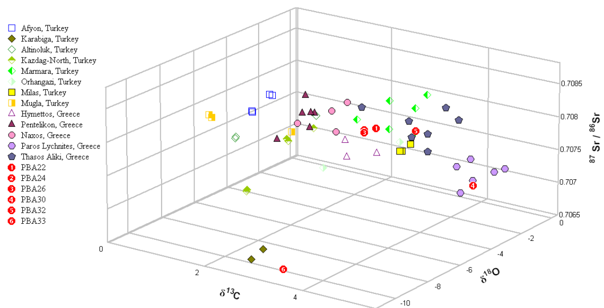
Figure 104: Trivariate method using \delta^{13}\text{C} , \delta^{18}\text{O} und ^{87}\text{Sr}/^{86}\text{Sr} isotopic results. The red numbers represent the marble objects of the Roman period of Troia.
