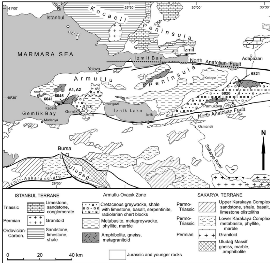
Figure 10: Geological map of the Armutlu-Ovacık Zone (after (OKAY et al. 2008)).
