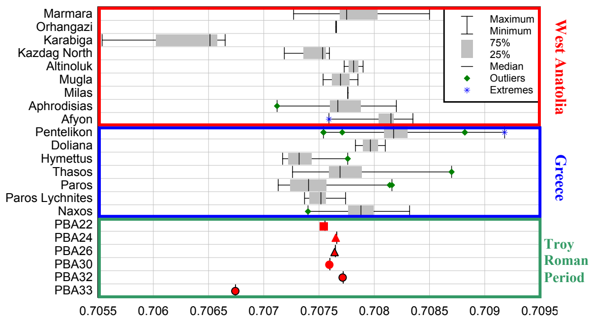
Figure 100: ^{87}\text{Sr}/^{86}\text{Sr} isotopic ratios of archaeological samples of the Roman Period of Troia compared with those from Anatolia and Greece (including data from PENTIA et al. 2002; ZÖLDFÖLDI & SATIR 2003; BRILLI et al. 2005).
