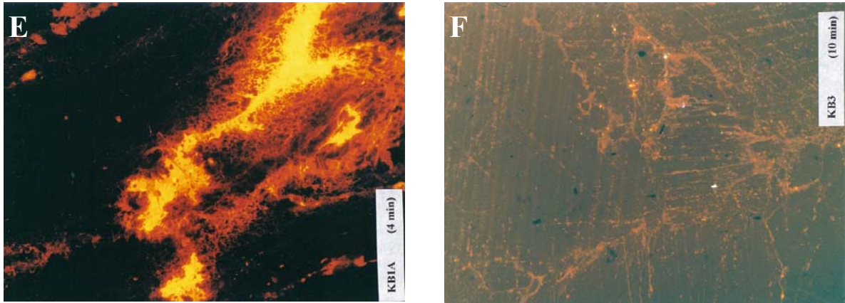
Figure 73: Typical CL patterns of marbles from Altınoluk (A), Bergaz (B), Marmara (C), Orhangazi (D) and Karabiga (E and F).
