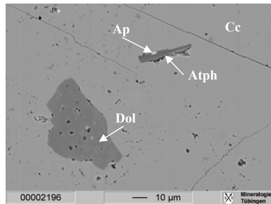
Figure 42: BSE image of sample M10. Calcitic matrix with dolomite (Dol), anthophyllite (Atph) and apatite (Ap).
