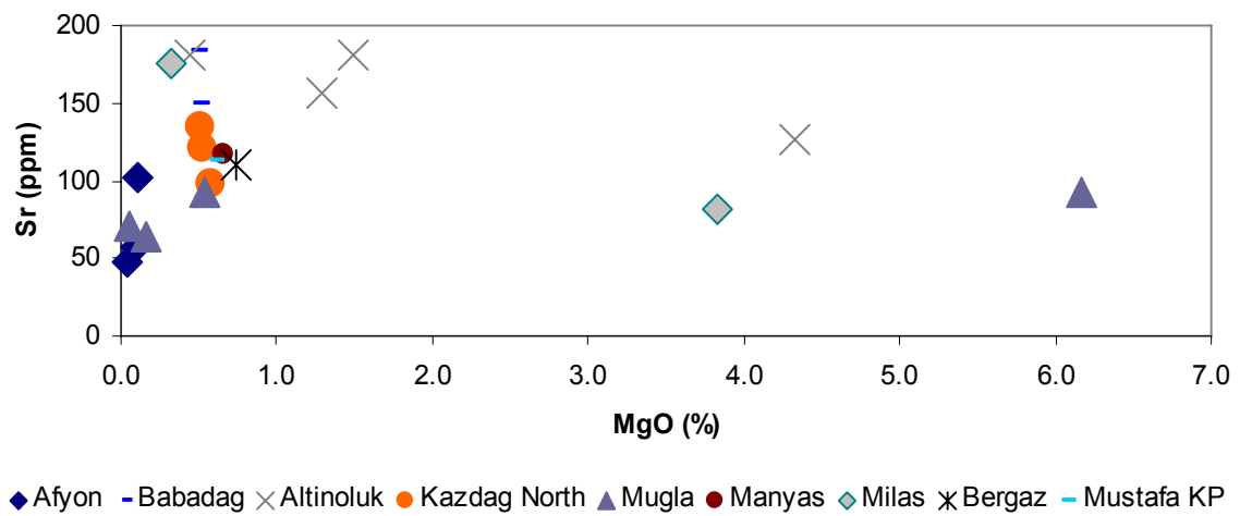
Figure 68: MgO vs. Sr bivariate plot, showing the differences of the chemical composition of the marble occurrences.
