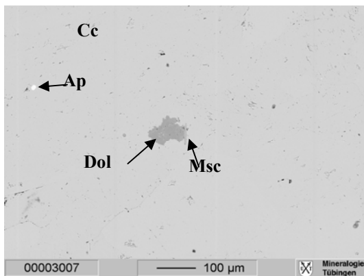
Figure 47: BSE image of sample PBA6. Calcitic marble with small amount of dolomite (Dol), muscovite (Msc) and apatite (Ap)
