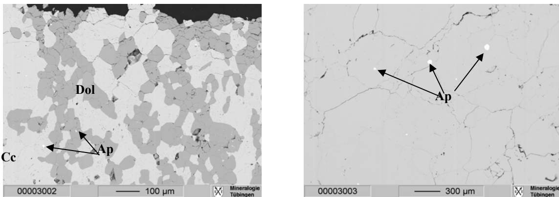
Figure 56: BSE image of sample PBA31. Marble with high amount of dolomite (Dol) and apatite crystals that are scattered throughout the sample.
