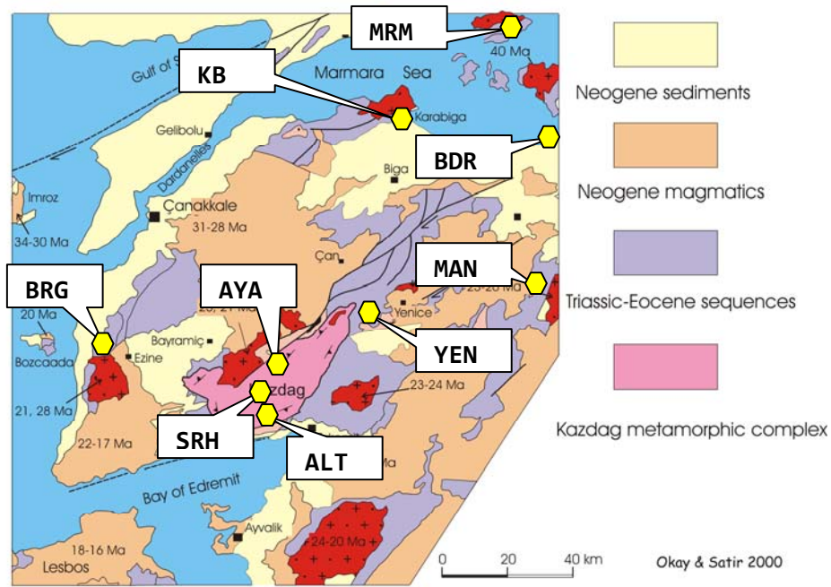
Figure 16: Simplified tectonic map of the Biga Peninsula (Okay & Satir 2000), NW-Turkey with sampled marble locations: KB = Karabiga, AYA = Ayazma, YEN = Yenice, BRG = Bergaz, SRH = Serhat, ALT = Altınoluk, MAN = Manyas, BDR = Bandırma, MRM = Marmara.
