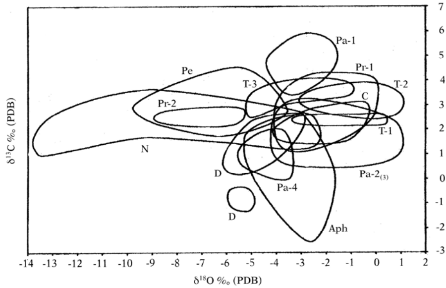
Figure 26: Stable isotopic database published by GORGONI et al. in 2002. Eight quarry sites subdivided into 11 groups are present in the database according the following abbreviations: Aph=Aphrodisias, C=Carrara, D=Docimium (Afyon), N=Naxos, Pa-1=Paros-Marathi or Lychnites, Pa-2=Paros Chorodaki, Pa-3=Paros-Haghios Minas, Pa-4 Paros Karavos, Pe=Pentelikon, Pr-1 and Pr-2 Proconnesos (Marmara), T-2=Thasos Aliki, T-3= Thasos Cape Vathy and Saliara (dolomitic marbles).
