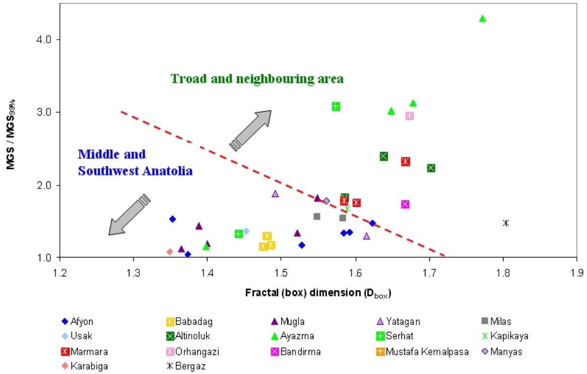
Figure 63: Cross plot of fractal dimension ( D_{box} ) vs. MGS/MGS_{99\%} . Note the separation line between the main geological units of West Anatolia.
