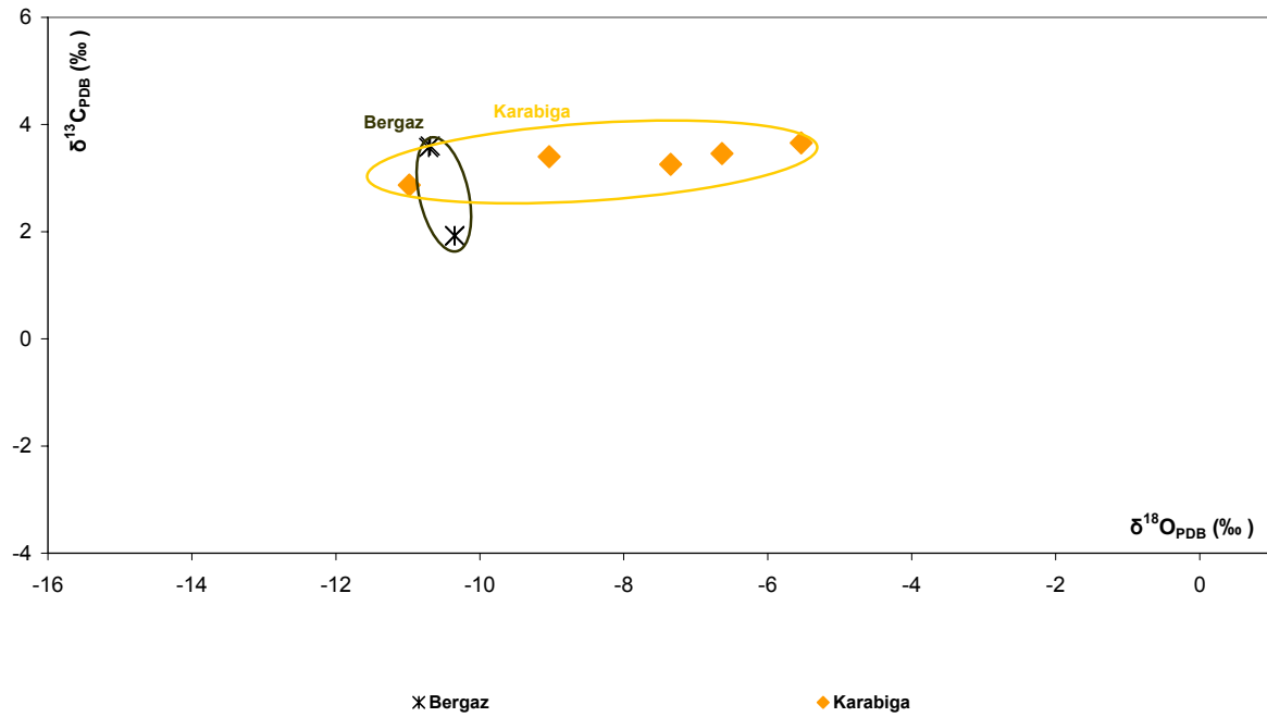
Figure 79: \delta^{13}\text{C} versus \delta^{18}\text{O} isotopic ratios (in ‰, relative to PDB) of the marble quarries belonging to the Rhodope-Strandja Massif in Northwest Anatolia. These measurements were carried out in the course of this work. No complementary data are available from these quarries.
