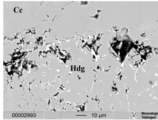
Figure 31: BSE image of the sample KB1A. Calcitic marble with hedenbergite (Hdg).
