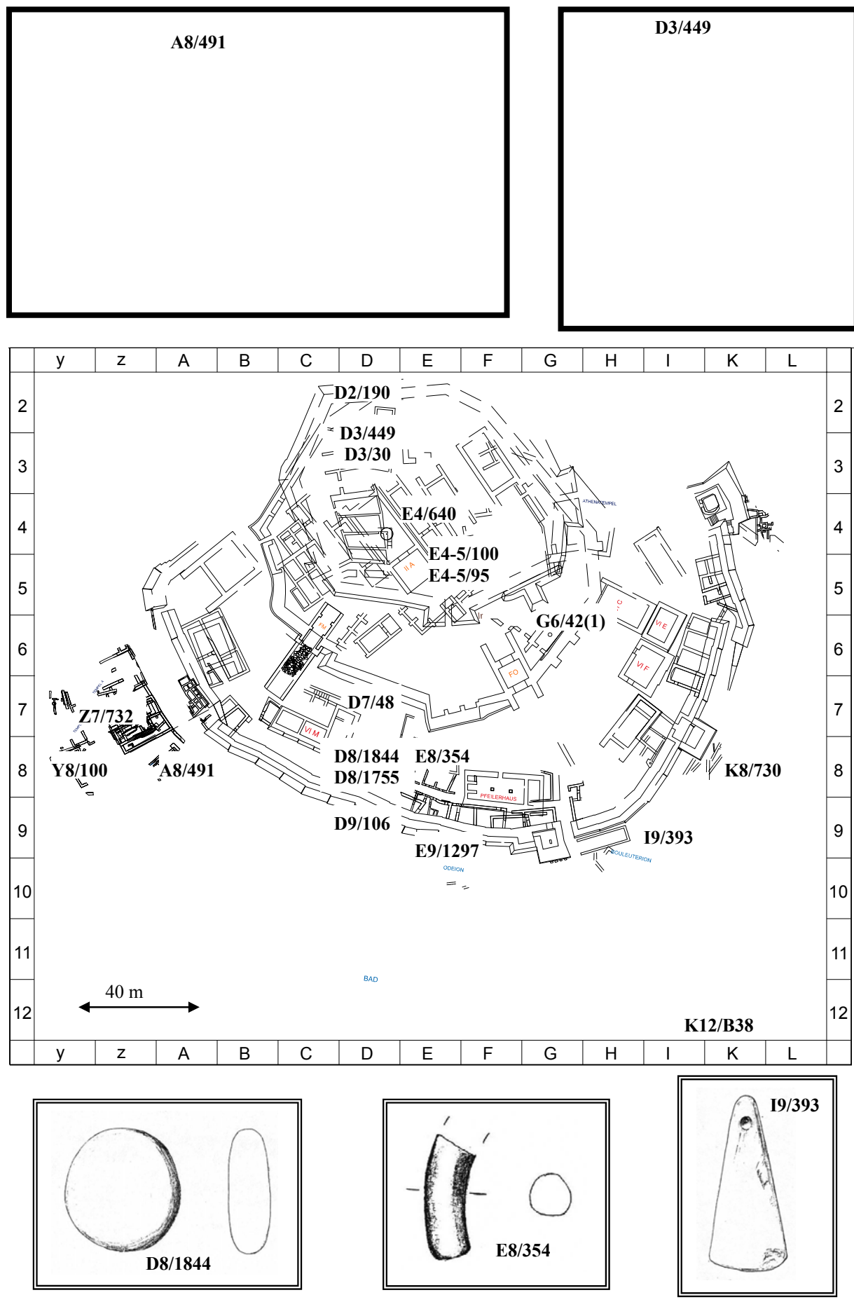
Figure 14: Plan of Troia I to VII with sampled of Bronze Age marble objects and drawings of some selected objects. (© Troia project)
