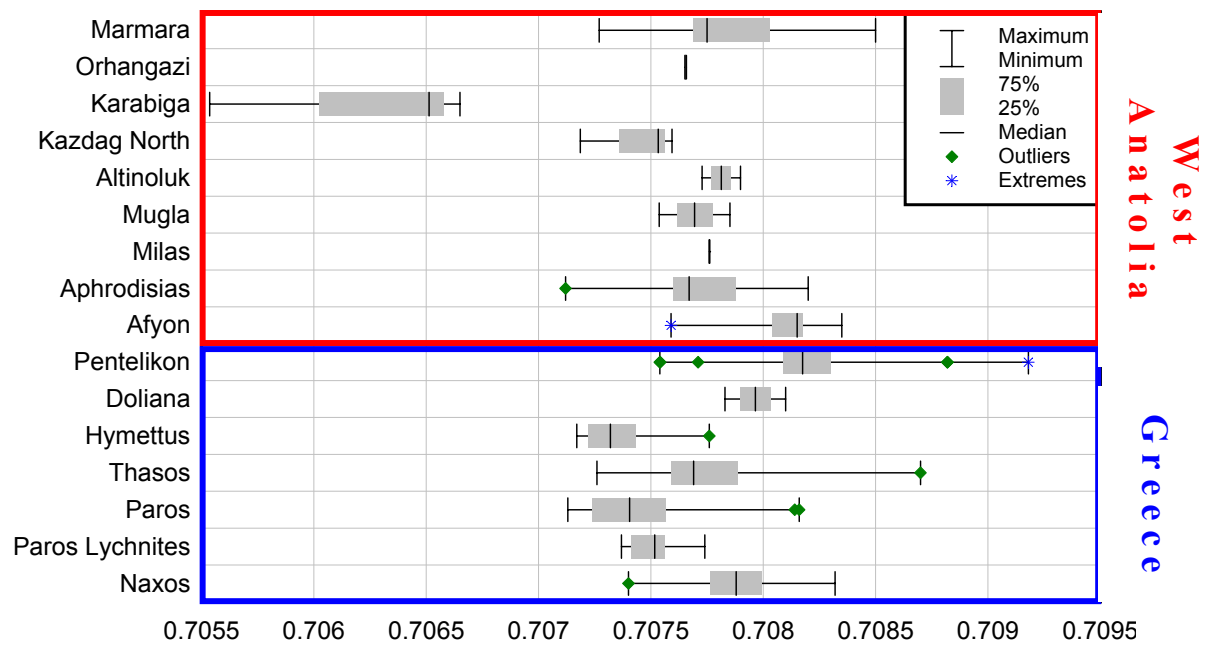
Figure 96: Distribution of the ^{87}\text{Sr}/^{86}\text{Sr} ratios of marbles from West Anatolia and Greece including data from BRILLI et al. (2005) and PENTIA et al. (2002).
